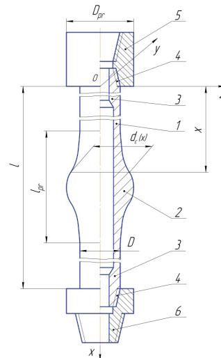
Fig. 4. General view of the developed design of aluminum drill pipe with a protector thickening of optimal shape: 1 – body of the pipe; 2 – protector thickening; 3 – inner near-end thickening; 4 – threaded connection; 5 – coupling of the drilling lock; 6 – nipple of the drilling lock
